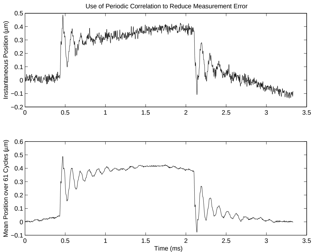
Figure 5-15: Reduction of noise through averaging. The top figure shows a single period of response to a 300 Hz square wave. The rms noise was measured to be 32 nm (DC to 100 kHz). The lower figure shows the mean response over 61 periods. The rms was calculated to be 4.1 nm.
