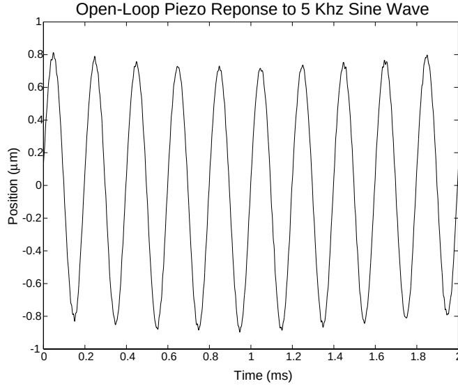
Figure 5-11: Open-loop piezo response to a 5 kHz sine wave. The system oscillated at 5 kHz. Additional low frequency vibrations can be seen in the envelope of the sinusoidal motion.
