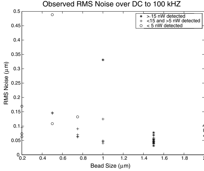
Figure 5-8: RMS noise with bead size for DC to 100 kHz.
