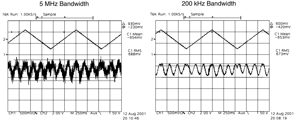
Figure 4-10: Demonstration of modulation. A 1\text{ }\mu\text{m} bead was linearly swept through a 10\text{ }\mu\text{m} range across a fringe pattern with approximately 3\text{ }\mu\text{m} spacing. The bead cycled at 0.9\text{ Hz} . When illuminated by a total of approximately 5\text{ mW} , modulation was evident at both 5\text{ MHz} (left) and 200\text{ kHz} (right) observation bandwidth.
