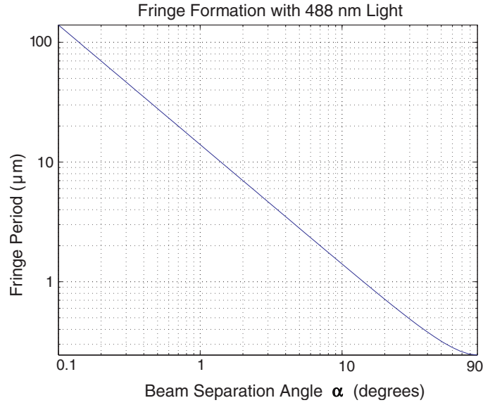
Figure 2-3: Fringe period with beam separation. The relation between fringe period and beam separation is shown for an index of refraction of 1 and rotation angle of 0 degrees.
