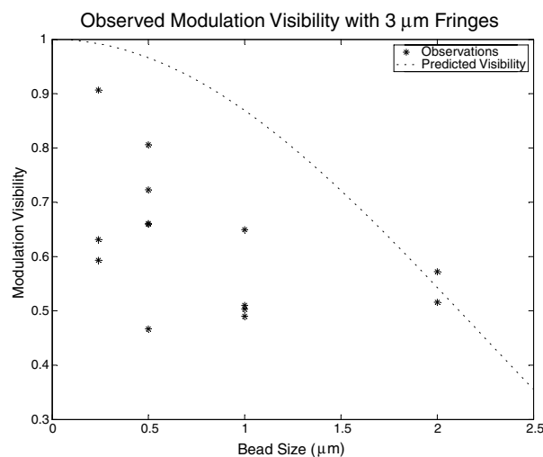
Figure 4-12: Measured modulation visibility. For each setup, a different ratio of output range to maximum output occurred. The dashed line shows the expected visibility based on isolated scattering by one disc in a fringe pattern. The data were taken from experiments with 3\ \mu\text{m} fringes and were measured at 1 MHz.
