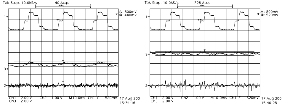
Figure 4-9: Out-of-line coupling. The piezo was swept through a 10\text{ }\mu\text{m} range of movement shown in top trace in both figures. The relative horizontally coupled motion is shown the left in the second trace while the vertical coupling motion is shown on right. In both cases out of plane movement was less than 1.6\text{ }\mu\text{m} (corresponding to 800 mV). The laser Doppler velocity readings for both positions are shown as the bottom traces.
